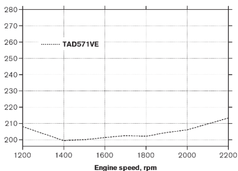
Fuel consumption, g/kWh
