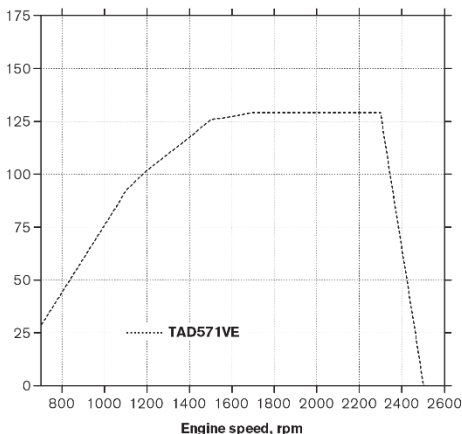
Power, kW
