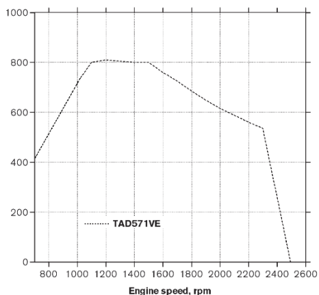
Torque, Nm
